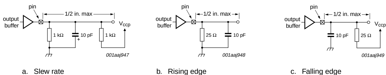
Fig 16. Type P cell test load conditions; see Table 18
