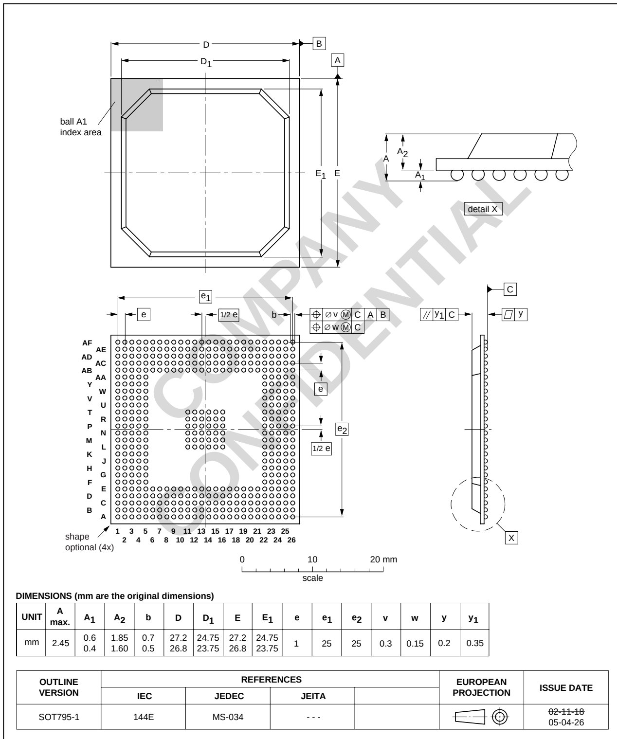
Fig 22. Package outline SOT795-1 (BGA456)
