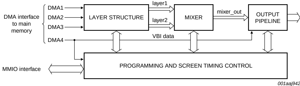
Fig 4. QVCP top level block diagram
