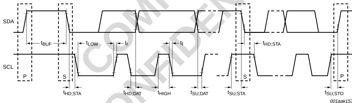
Fig 20. I 2 C-bus interface timing
